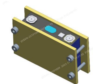
Fig. 4 Side view of battery shaft 图 4 电池轴测图
