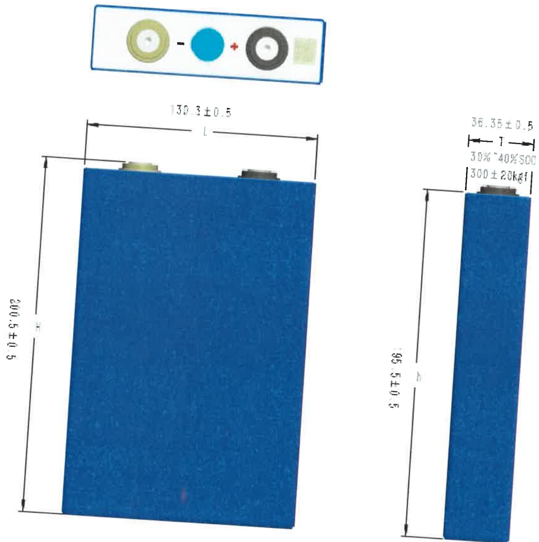
Fig.7 Cell Drawing of LF105
