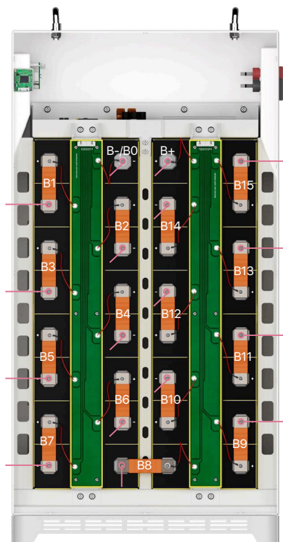
Linking Equalizer Cables (J)
